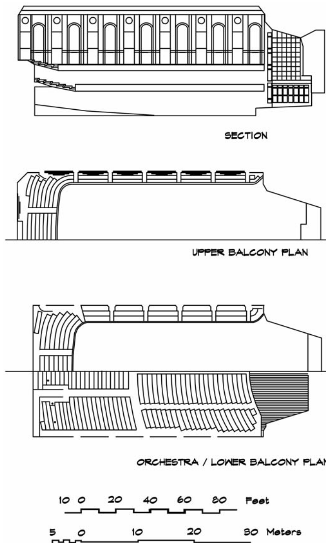
Fig. 2. Symphony Hall, Boston, Massachusetts, United States of America (Beranek, 1996).
