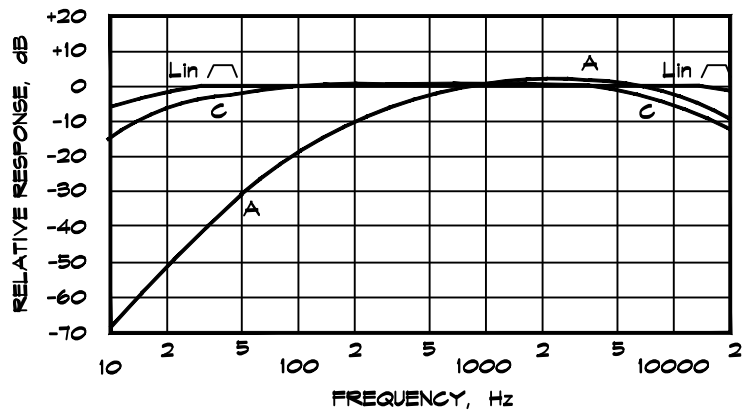
FIGURE 4.12 A, C, and Lin \wedge Weighting Characteristics (Bruel and Kjaer, 1979)
