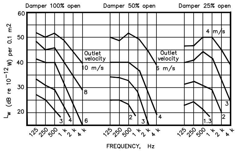
FIGURE 13.25 Ceiling Diffuser Damper - Sound Power Level (Fry, 1988) 1 m/sec = 196.8 ft/min
